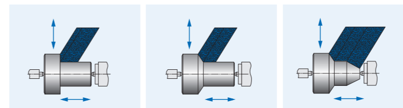
EXTERNAL ANGULAR PLUNGE GRINDING WITH EJ 11, EJ 31 AND EJ 51
